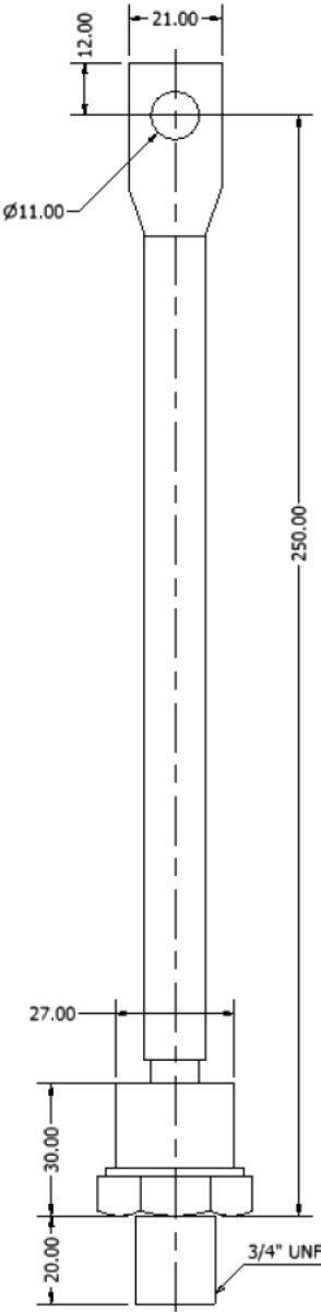
ALL DIMENSIONS IN MM
